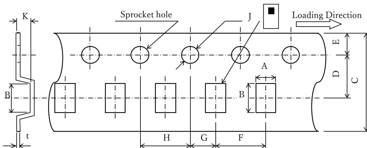
Carrier Tape
