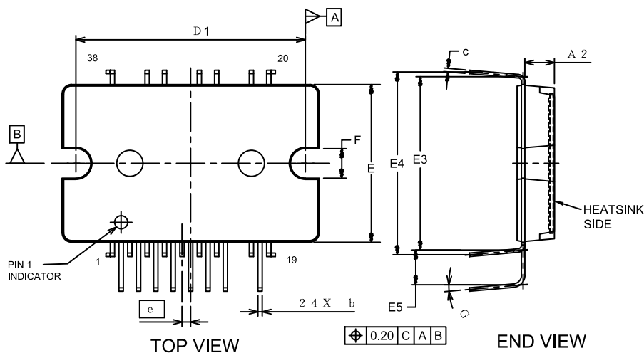
DIP38 29.60x18.20 EP-5 CASE 181AE ISSUE A
