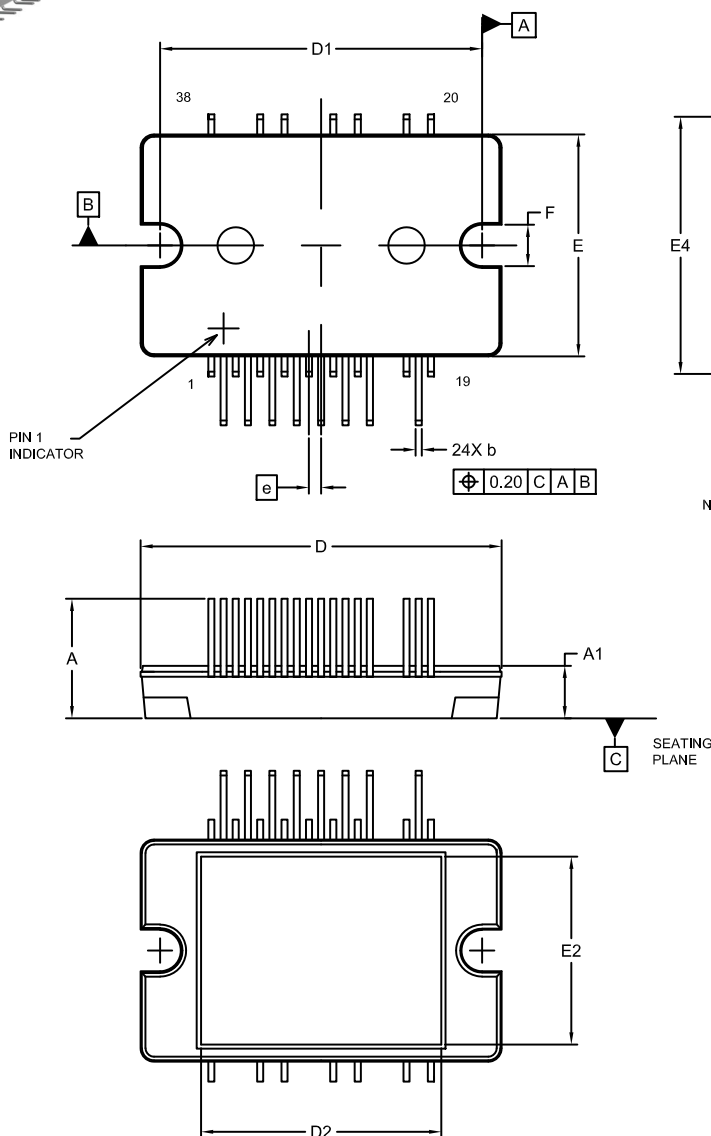
DIP38, 29.6x18.2 EP-3 CASE 125BT ISSUE A
